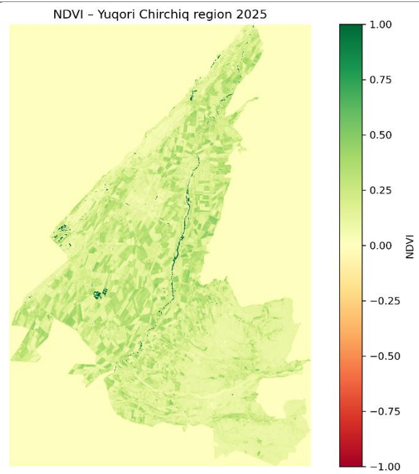
Figure 7. Spatial distribution of the NDVI index and vegetation classification in 2025.
