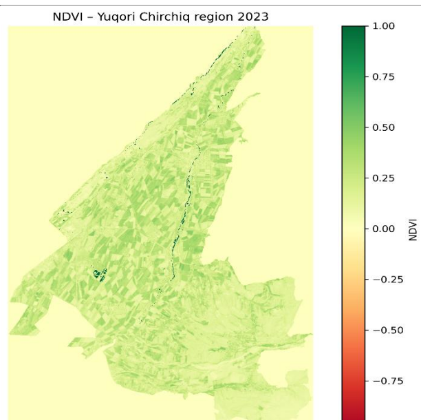
Figure 5. Spatial distribution of the NDVI index and vegetation classification in 2023.
